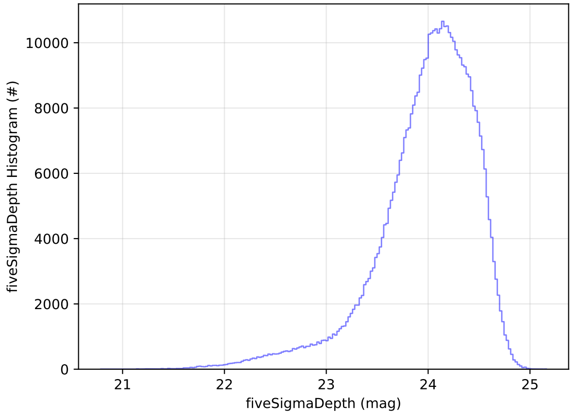
roll_uniform_eh_acc0.5_mjdp0_v3.4_10yrs All sky r band: fiveSigmaDepth Histogram
