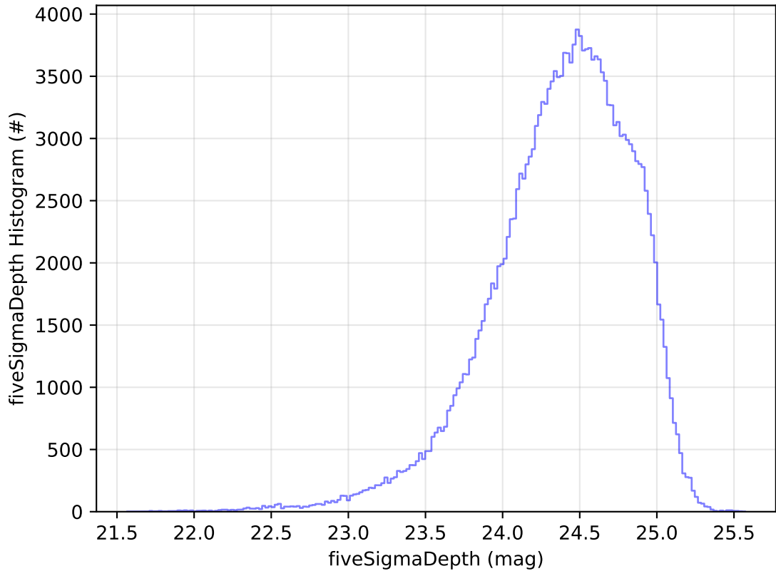
roll_uniform_eh_acc0.5_mjdp0_v3.4_10yrs All sky g band: fiveSigmaDepth Histogram
