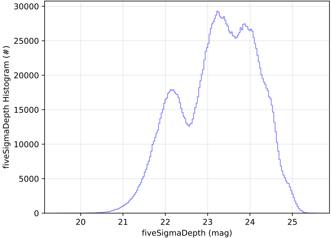
roll_uniform_eh_acc0.5_mjdp0_v3.4_10yrs All sky all bands: fiveSigmaDepth Histogram
