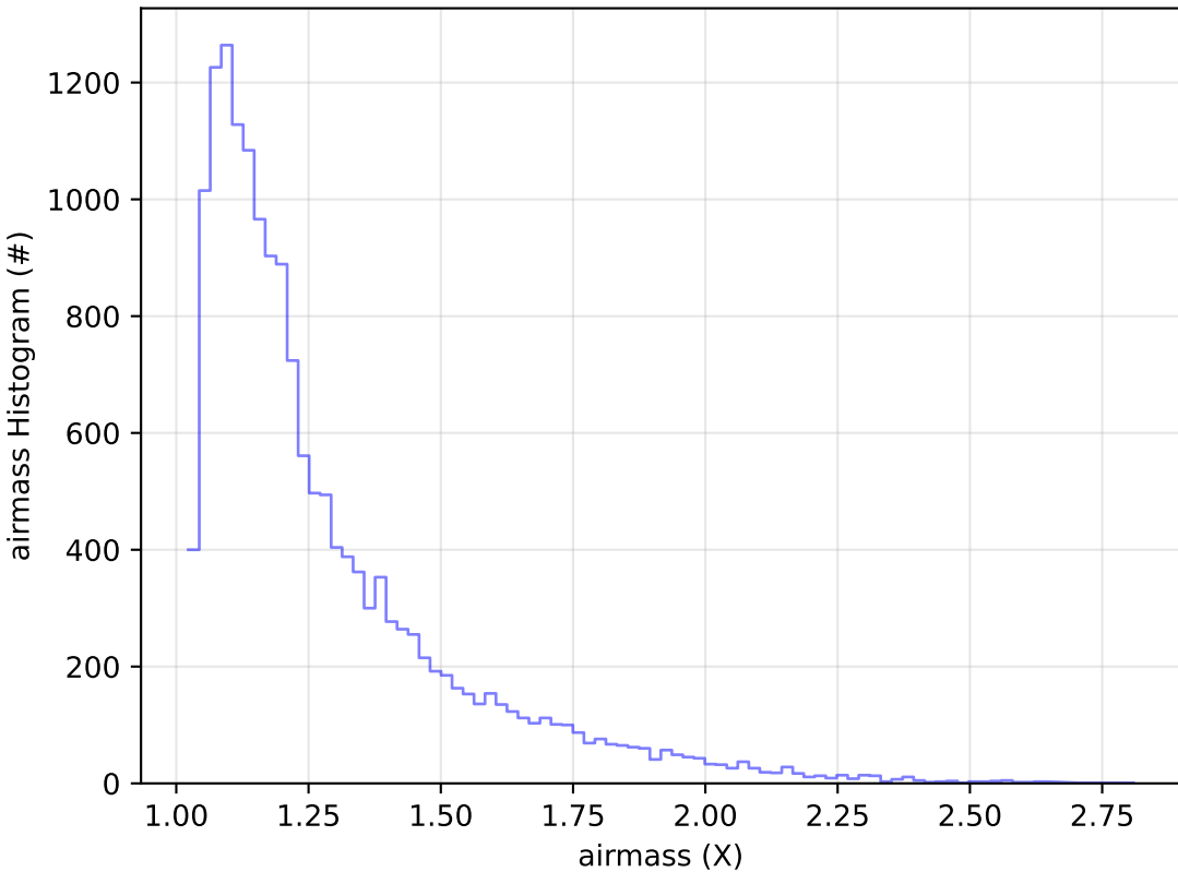
roll_uniform_eh_acc0.5_mjdp0_v3.4_10yrs Yr 1 u band: airmass Histogram
