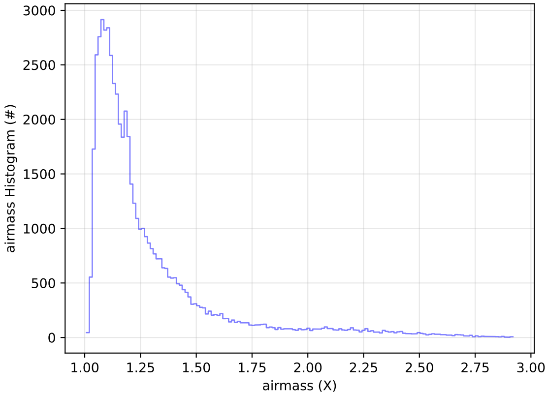
roll_uniform_eh_acc0.5_mjdp0_v3.4_10yrs Yr 1 i band: airmass Histogram
