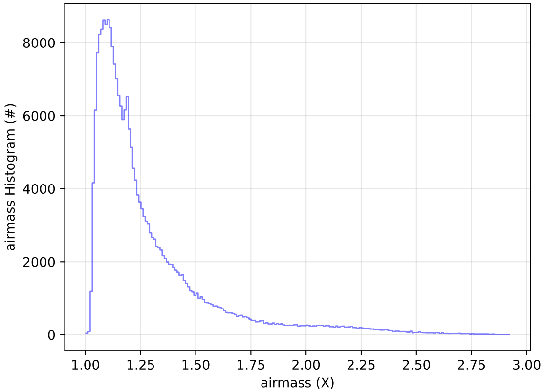
roll_uniform_eh_acc0.5_mjdp0_v3.4_10yrs Yr 1 all bands: airmass Histogram
