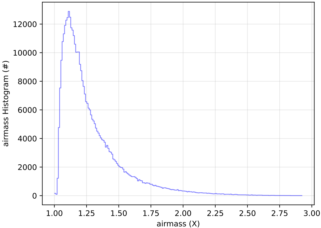
roll_uniform_eh_acc0.5_mjdp0_v3.4_10yrs WFD y band: airmass Histogram
