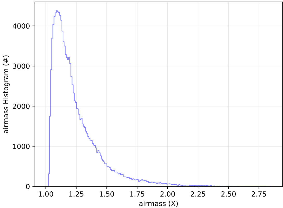
roll_uniform_eh_acc0.5_mjdp0_v3.4_10yrs WFD u band: airmass Histogram
