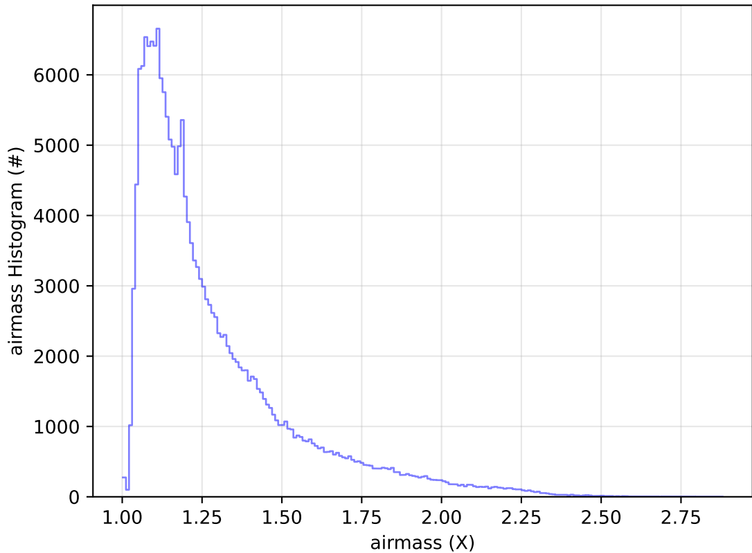
roll_uniform_eh_acc0.5_mjdp0_v3.4_10yrs WFD g band: airmass Histogram
