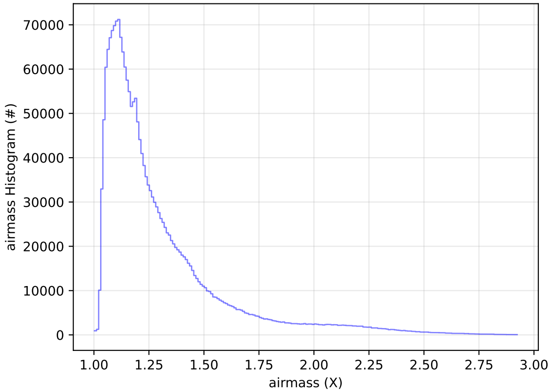
roll_uniform_eh_acc0.5_mjdp0_v3.4_10yrs WFD all bands: airmass Histogram
