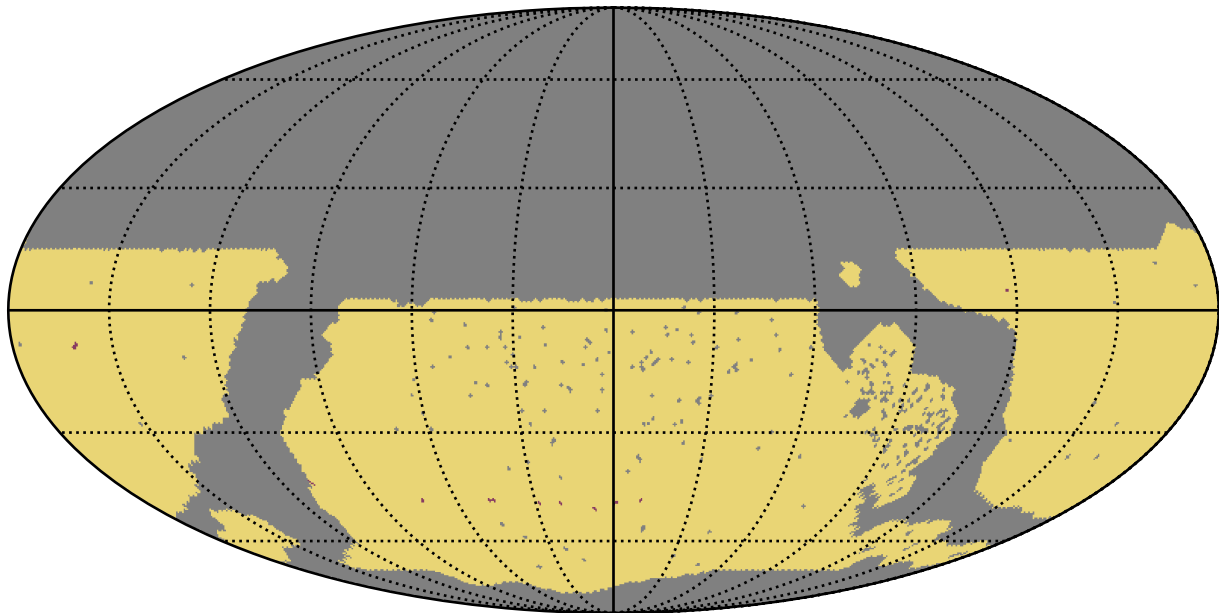
roll_uniform_eh_acc0.5_mjdp0_v3.4_10yrs WFD: RapidRevisits
