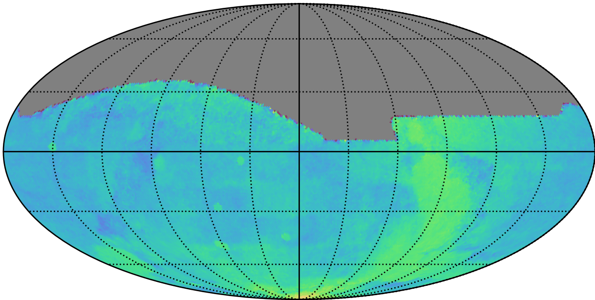
roll_uniform_eh_acc0.5_mjdp0_v3.4_10yrs All sky: Parallax Coverage @ 22.4
