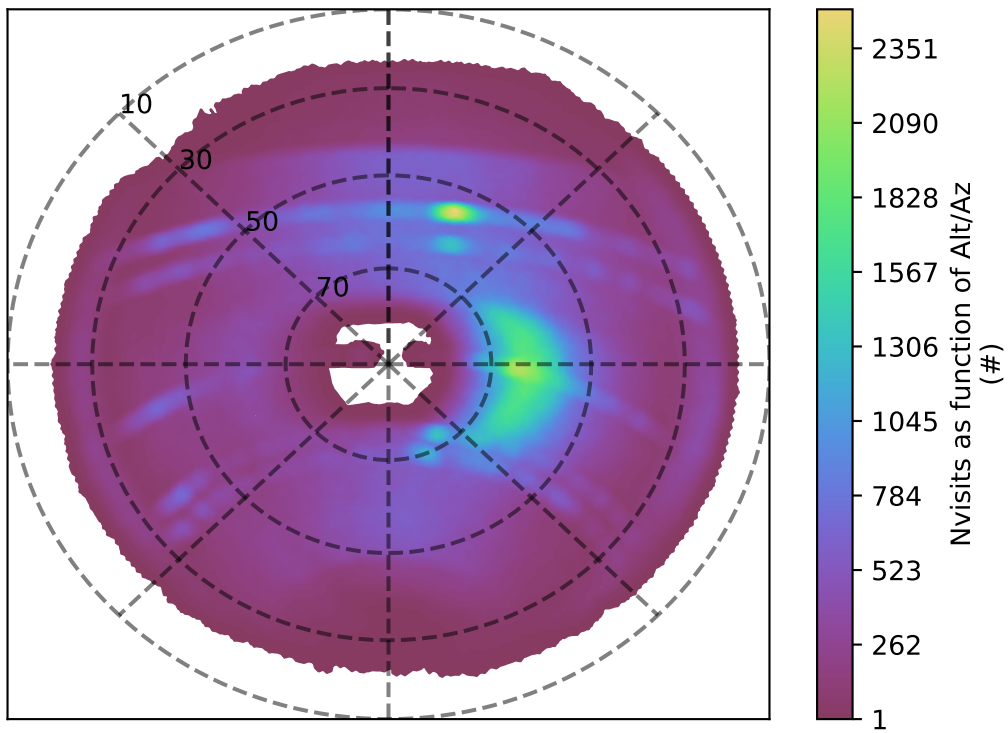
roll_uniform_eh_acc0.5_mjdp0_v3.4_10yrs z band: Nvisits as function of Alt/Az
