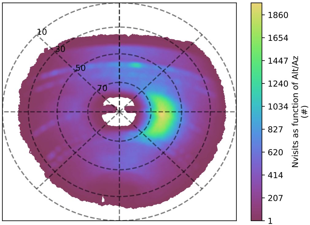
roll_uniform_eh_acc0.5_mjdp0_v3.4_10yrs y band: Nvisits as function of Alt/Az
