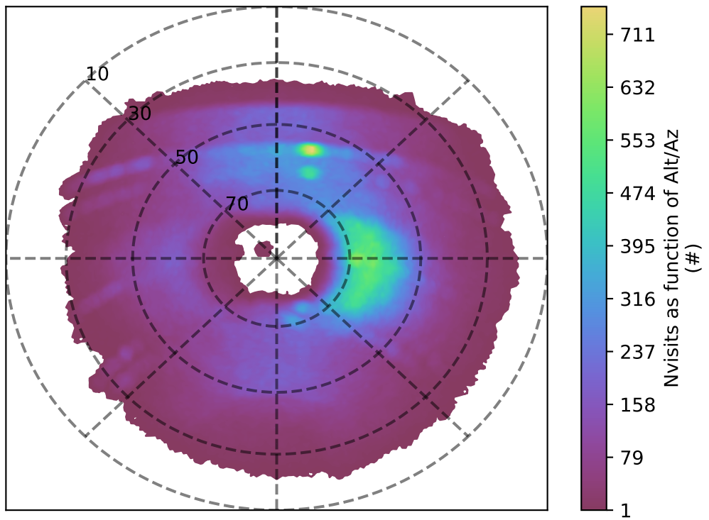
roll_uniform_eh_acc0.5_mjdp0_v3.4_10yrs u band: Nvisits as function of Alt/Az
