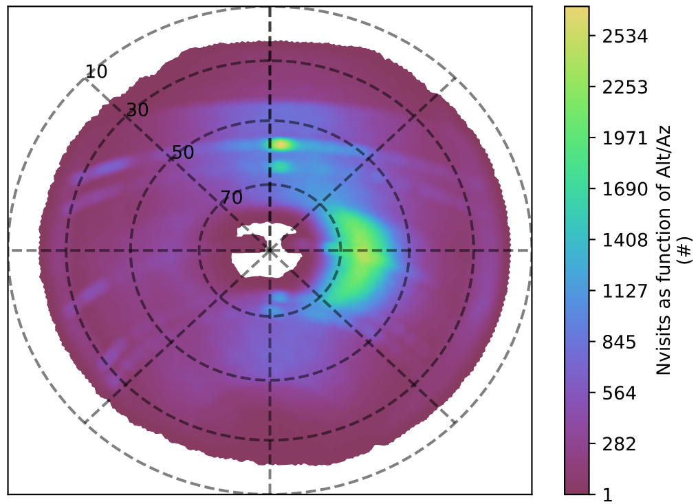
roll_uniform_eh_acc0.5_mjdp0_v3.4_10yrs i band: Nvisits as function of Alt/Az
