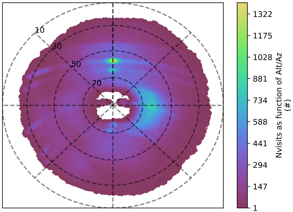
roll_uniform_eh_acc0.5_mjdp0_v3.4_10yrs g band: Nvisits as function of Alt/Az
