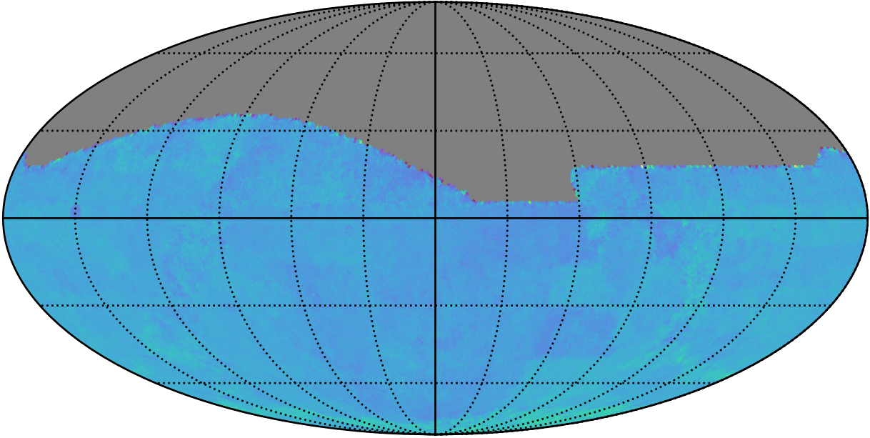
roll_uniform_eh_acc0.5_mjdp0_v3.4_10yrs All sky: Normalized Proper Motion Uncert @ 24.0
