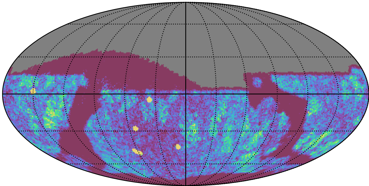
roll_uniform_eh_acc0.5_mjdp0_v3.4_10yrs Yr 1 z band: NVisits
