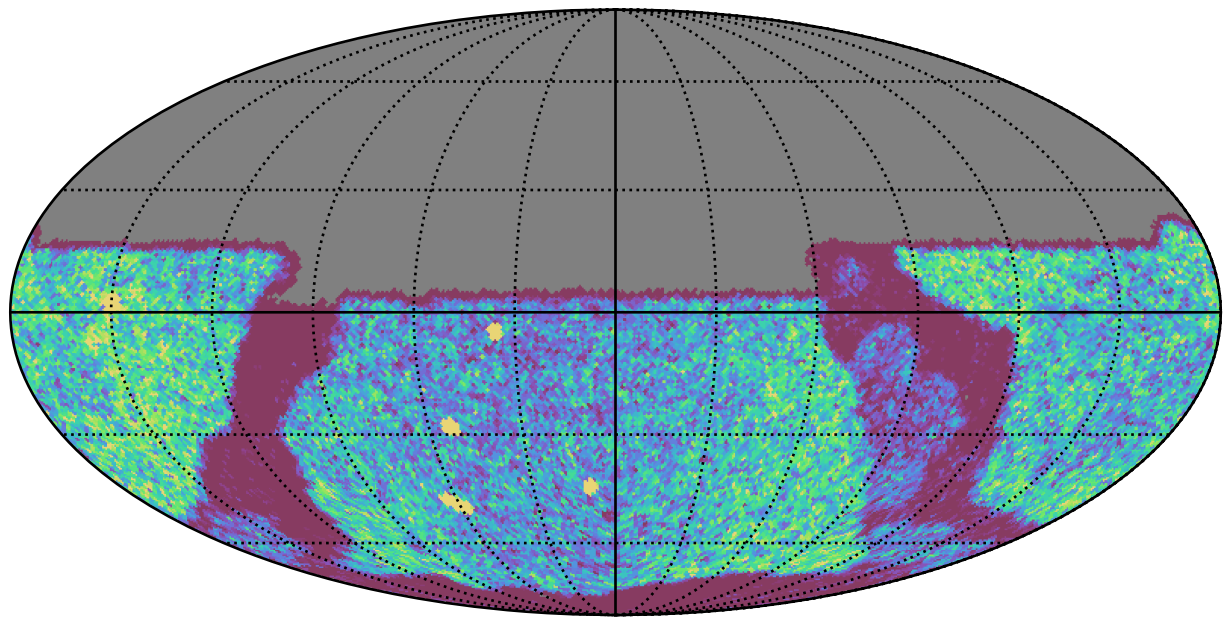
roll_uniform_eh_acc0.5_mjdp0_v3.4_10yrs Yr 1 y band: NVisits
