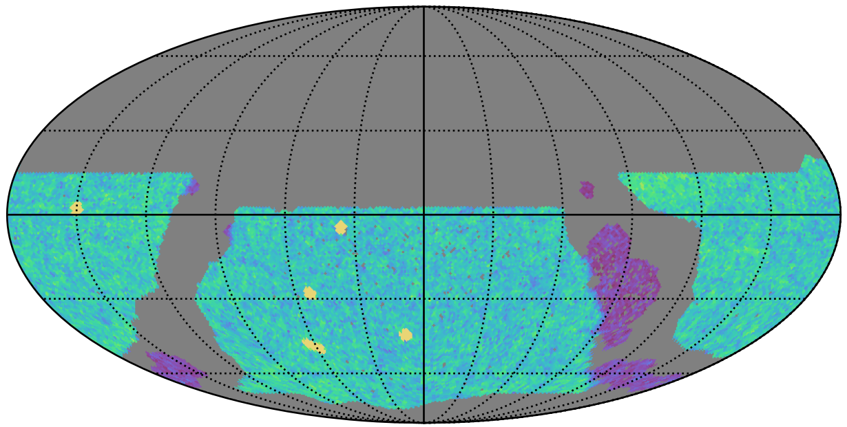
roll_uniform_eh_acc0.5_mjdp0_v3.4_10yrs WFD u band: NVisits
