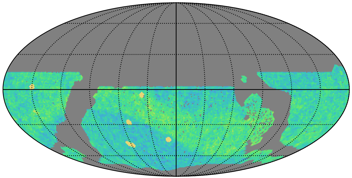
roll_uniform_eh_acc0.5_mjdp0_v3.4_10yrs WFD i band: NVisits
