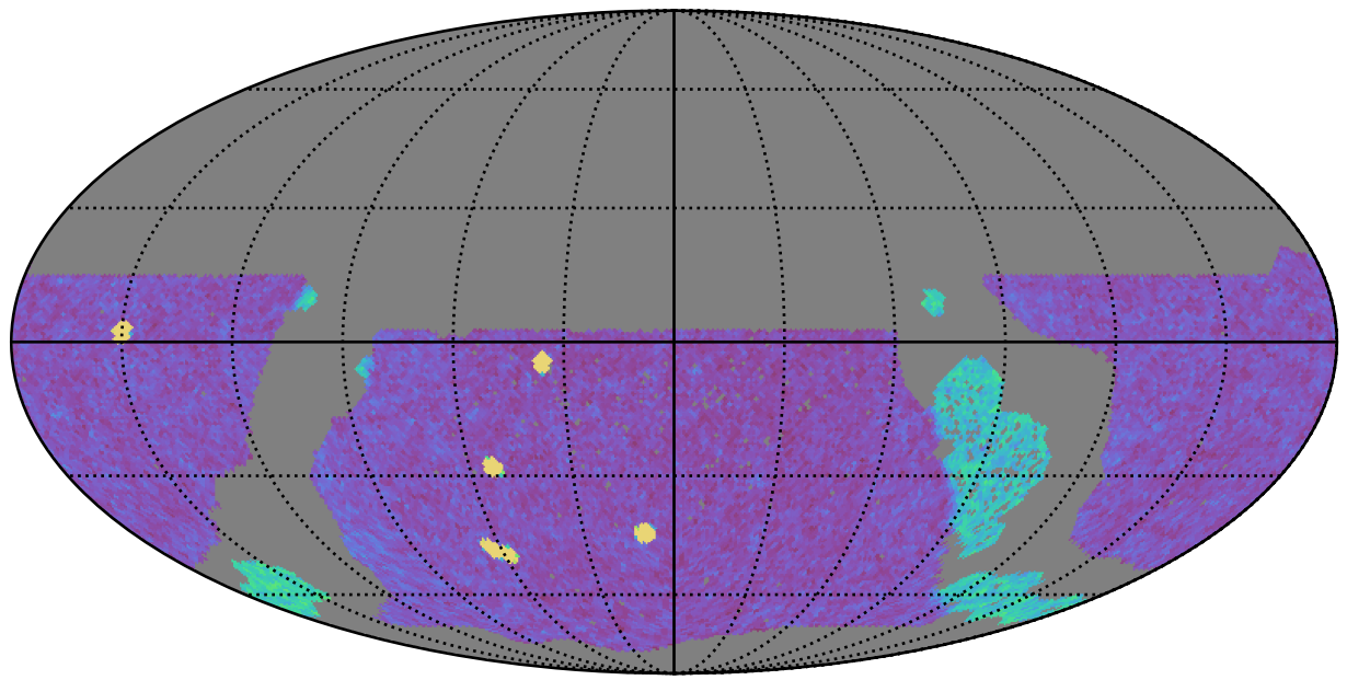
roll_uniform_eh_acc0.5_mjdp0_v3.4_10yrs WFD g band: NVisits
