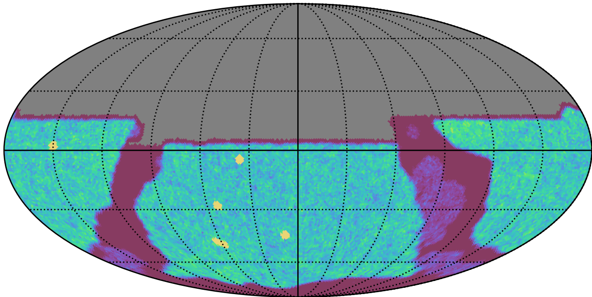
roll_uniform_eh_acc0.5_mjdp0_v3.4_10yrs All sky u band: NVisits
