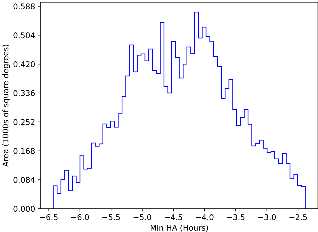
roll_uniform_eh_acc0.5_mjdp0_v3.4_10yrs WFD i band: Min HA
