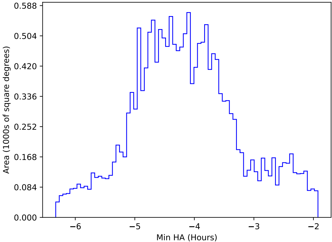
roll_uniform_eh_acc0.5_mjdp0_v3.4_10yrs WFD g band: Min HA
