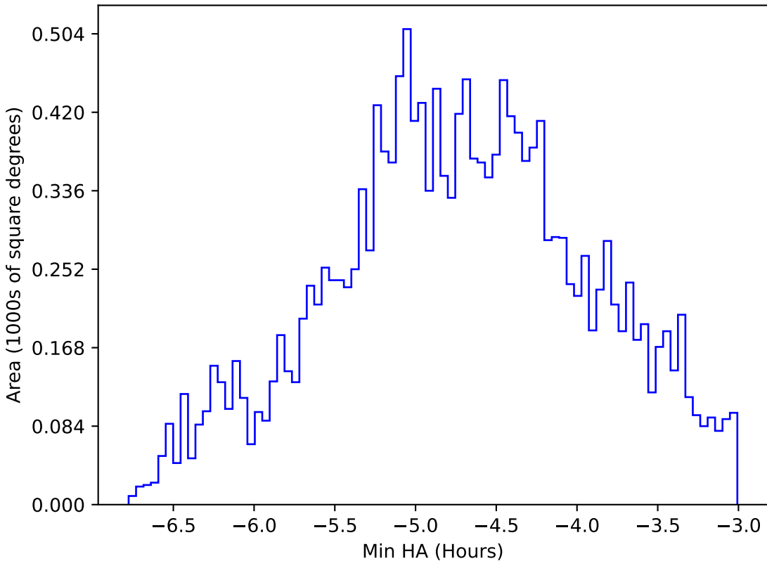
roll_uniform_eh_acc0.5_mjdp0_v3.4_10yrs WFD all bands: Min HA
