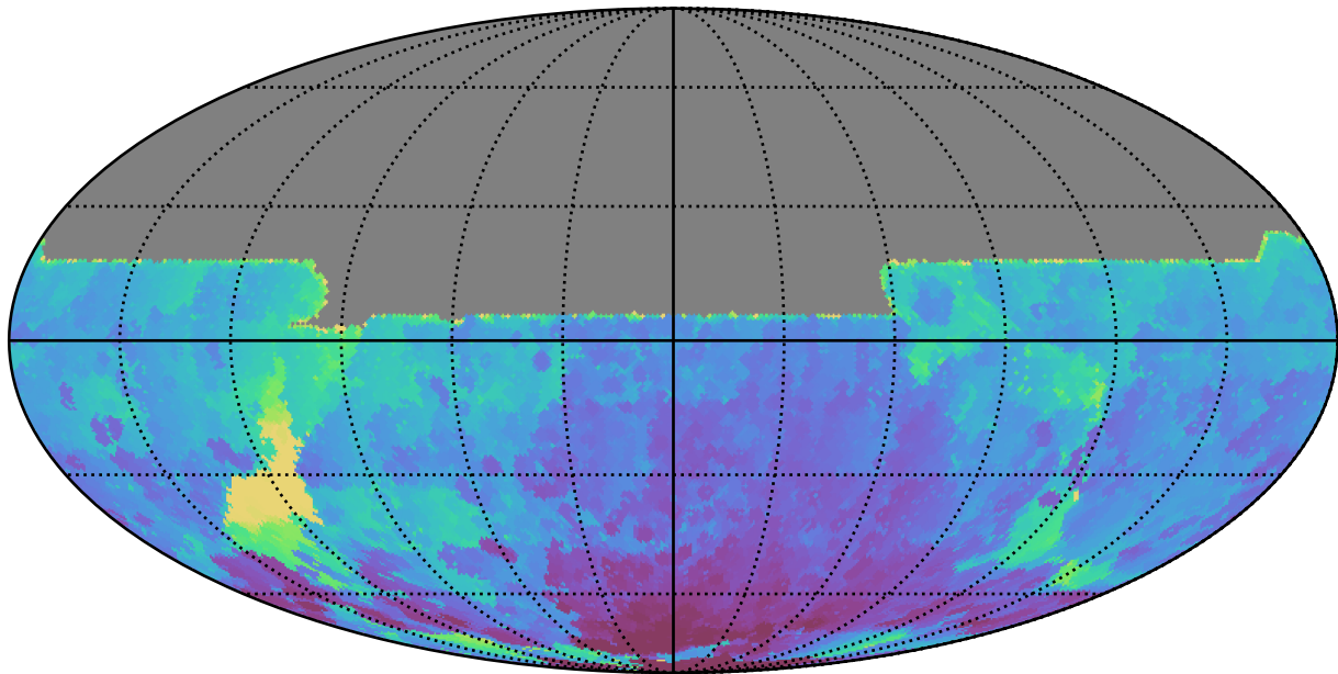
roll_uniform_eh_acc0.5_mjdp0_v3.4_10yrs All sky y band: Min HA
