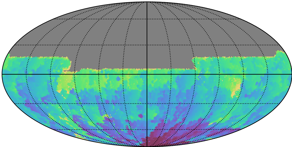
roll_uniform_eh_acc0.5_mjdp0_v3.4_10yrs All sky u band: Min HA
