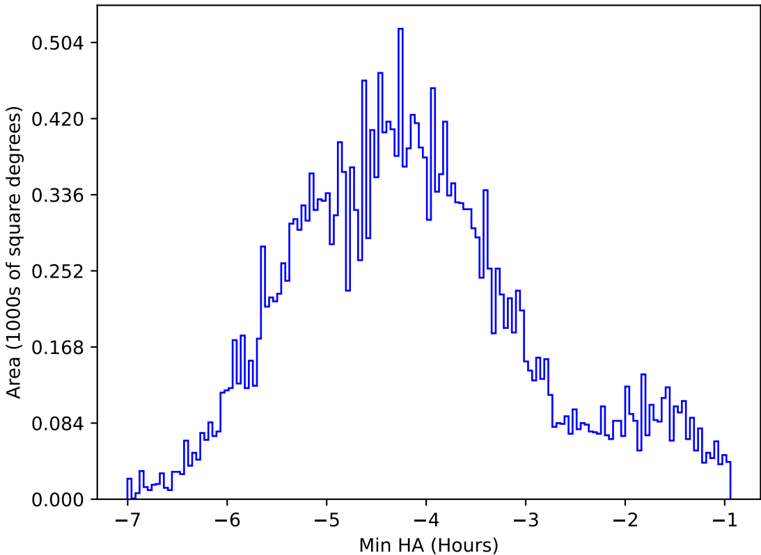
roll_uniform_eh_acc0.5_mjdp0_v3.4_10yrs All sky r band: Min HA
