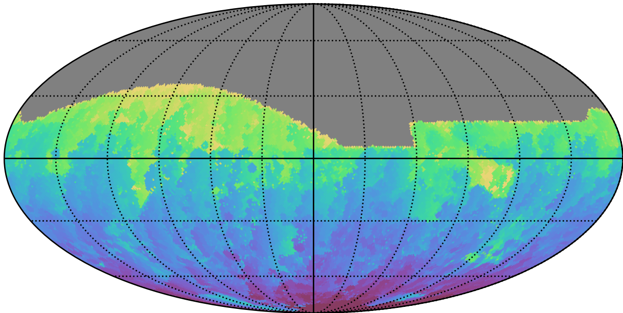
roll_uniform_eh_acc0.5_mjdp0_v3.4_10yrs All sky g band: Min HA
