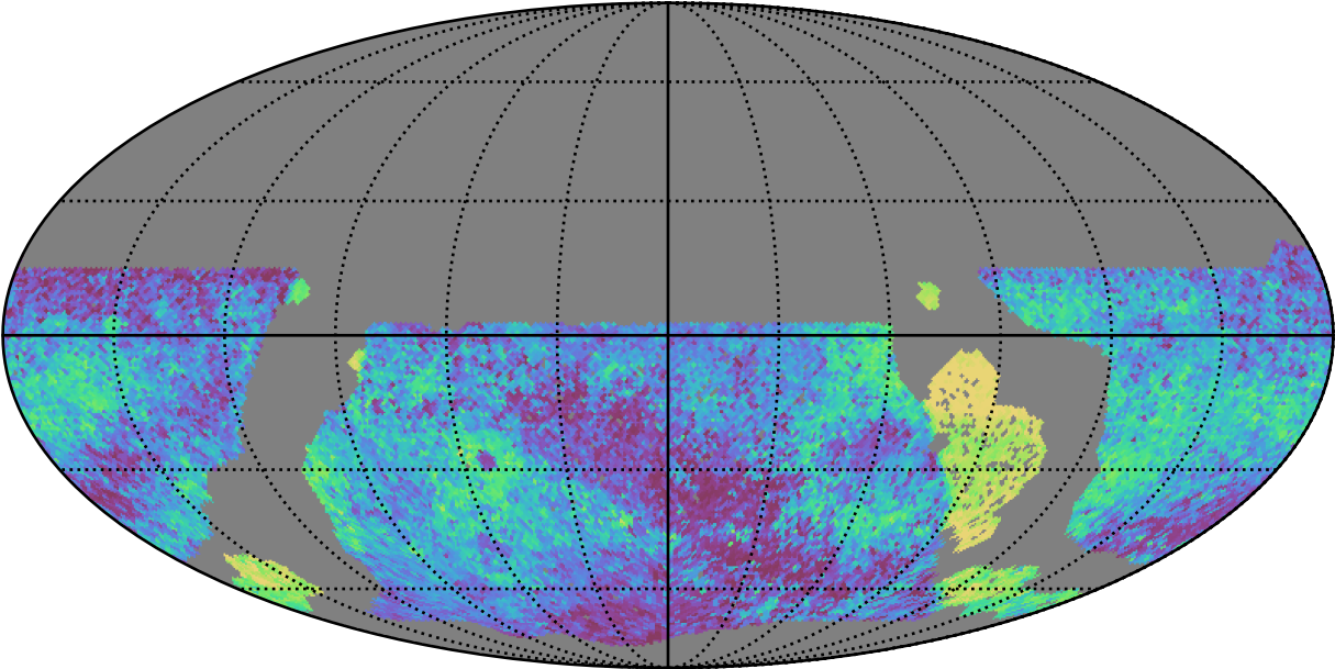
roll_uniform_eh_acc0.5_mjdp0_v3.4_10yrs WFD all bands: Median skyBrightness
