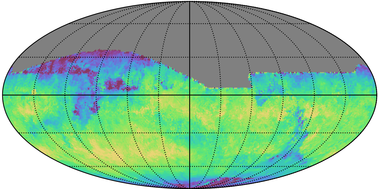
roll_uniform_eh_acc0.5_mjdp0_v3.4_10yrs All sky z band: Median skyBrightness
