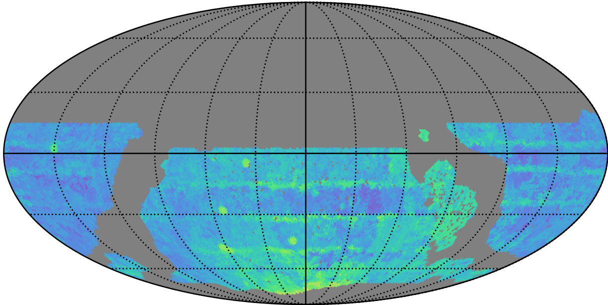
roll_uniform_eh_acc0.5_mjdp0_v3.4_10yrs WFD z band: Median Season Length
