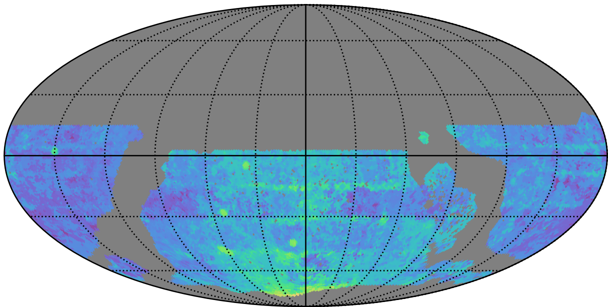
roll_uniform_eh_acc0.5_mjdp0_v3.4_10yrs WFD y band: Median Season Length
