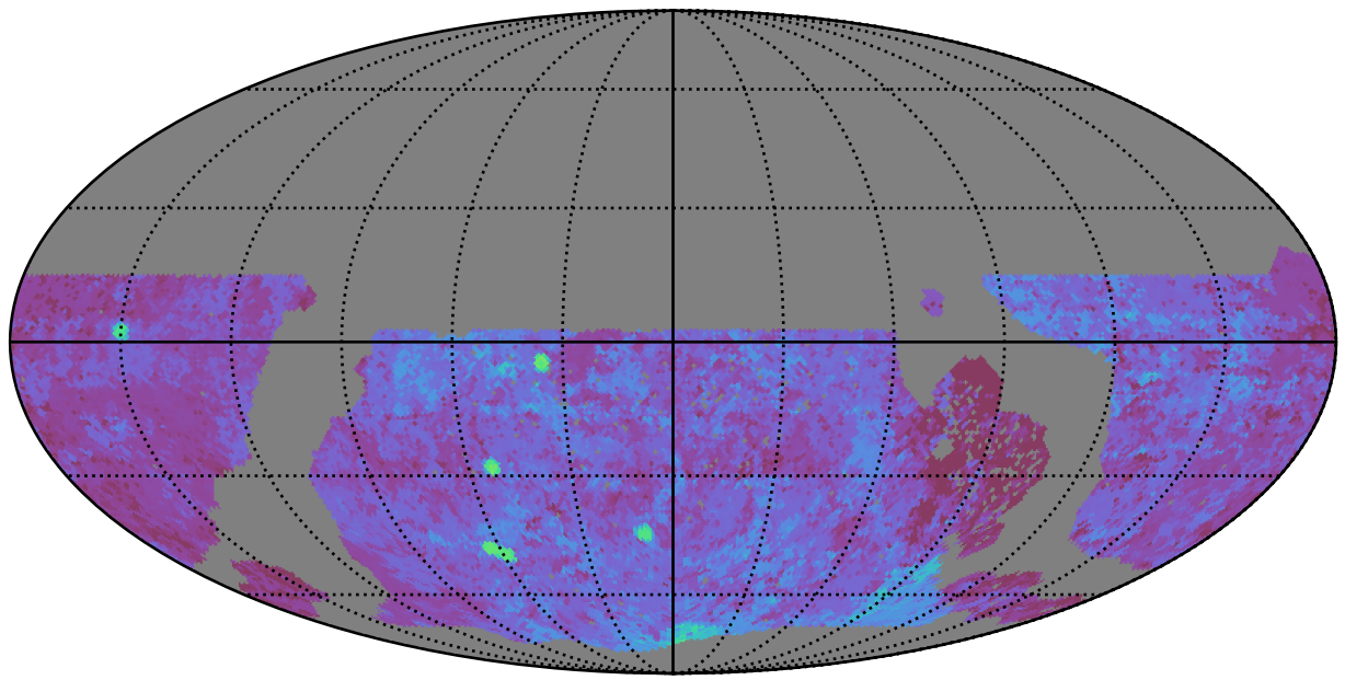
roll_uniform_eh_acc0.5_mjdp0_v3.4_10yrs WFD u band: Median Season Length
