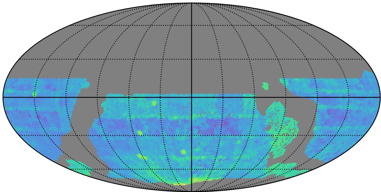
roll_uniform_eh_acc0.5_mjdp0_v3.4_10yrs WFD i band: Median Season Length
