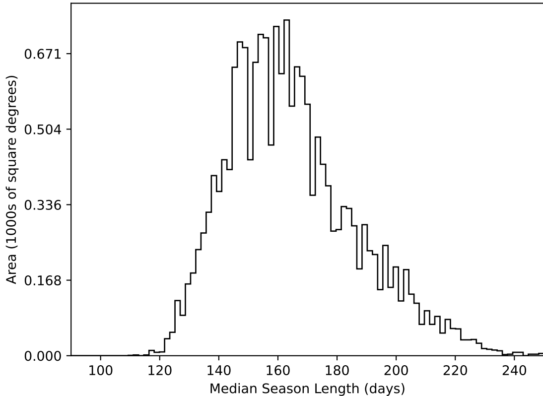
roll_uniform_eh_acc0.5_mjdp0_v3.4_10yrs WFD all bands: Median Season Length
