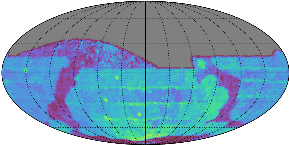
roll_uniform_eh_acc0.5_mjdp0_v3.4_10yrs All sky z band: Median Season Length
