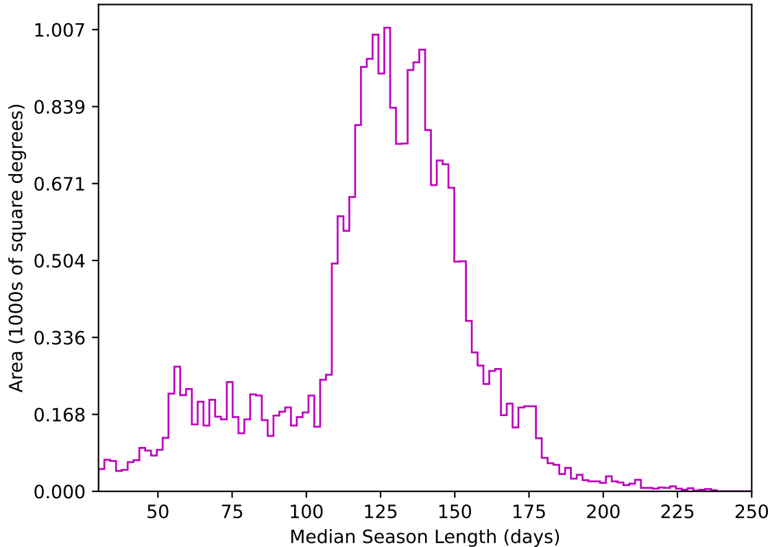
roll_uniform_eh_acc0.5_mjdp0_v3.4_10yrs All sky z band: Median Season Length
