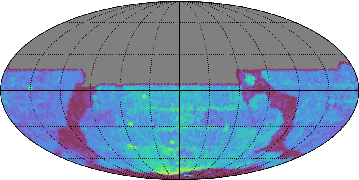
roll_uniform_eh_acc0.5_mjdp0_v3.4_10yrs All sky y band: Median Season Length
