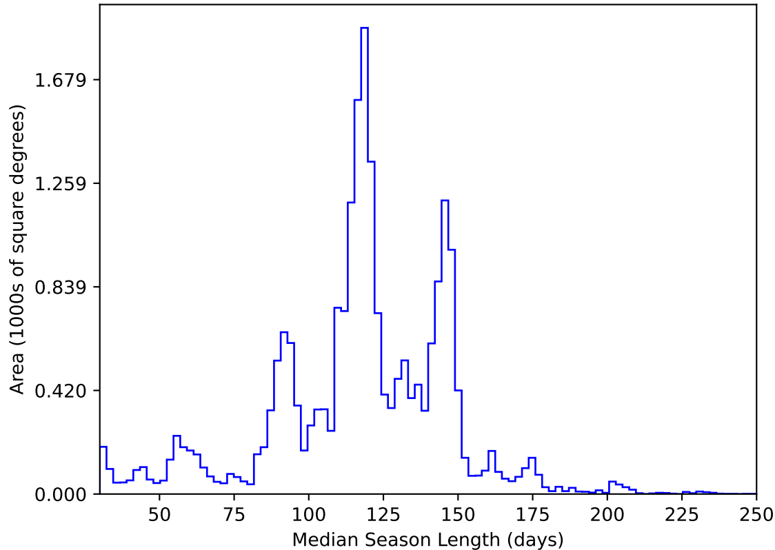
roll_uniform_eh_acc0.5_mjdp0_v3.4_10yrs All sky y band: Median Season Length
