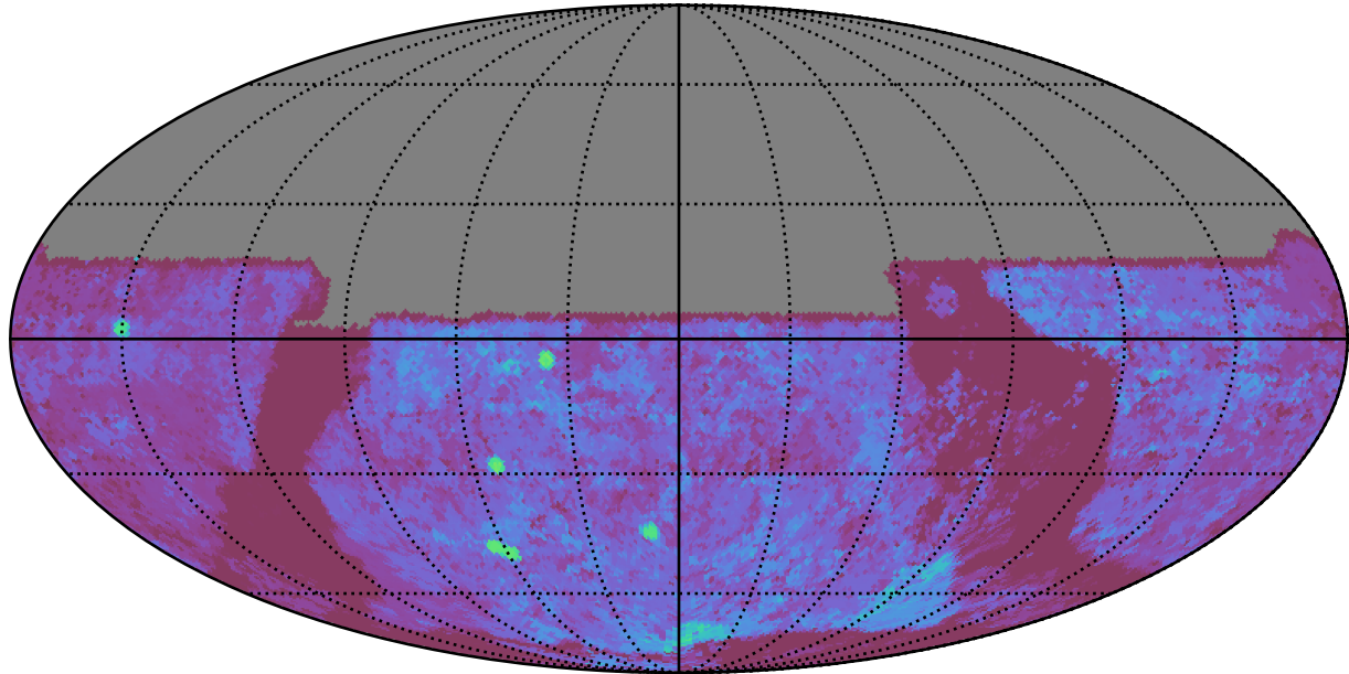
roll_uniform_eh_acc0.5_mjdp0_v3.4_10yrs All sky u band: Median Season Length
