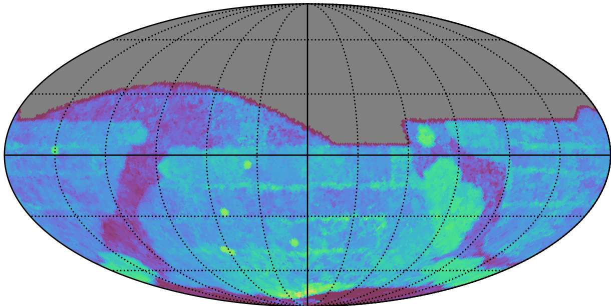
roll_uniform_eh_acc0.5_mjdp0_v3.4_10yrs All sky r band: Median Season Length
