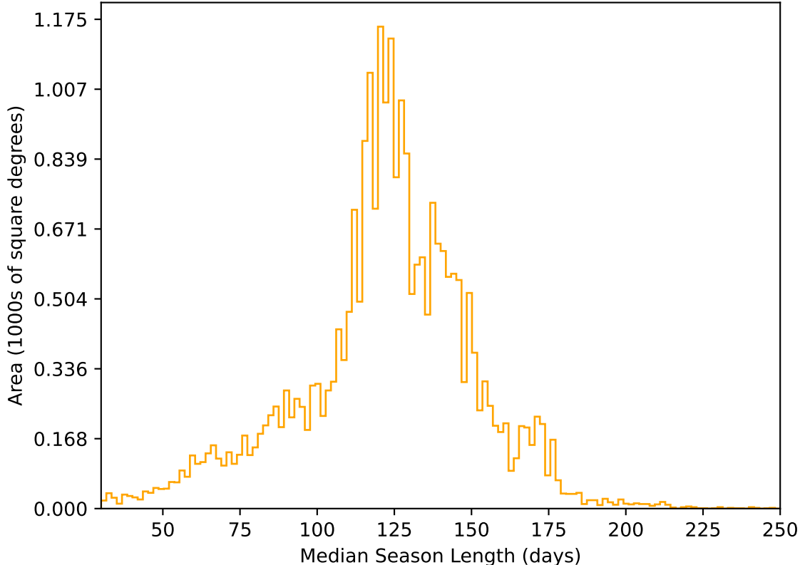
roll_uniform_eh_acc0.5_mjdp0_v3.4_10yrs All sky r band: Median Season Length
