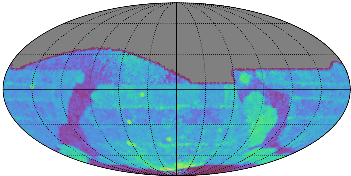
roll_uniform_eh_acc0.5_mjdp0_v3.4_10yrs All sky i band: Median Season Length
