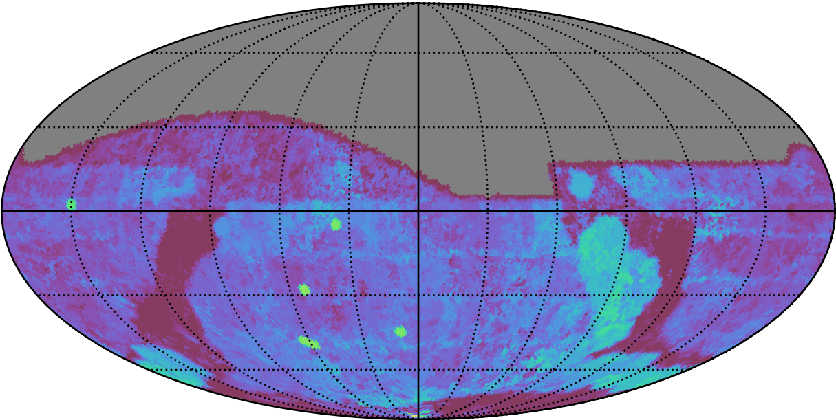
roll_uniform_eh_acc0.5_mjdp0_v3.4_10yrs All sky g band: Median Season Length
