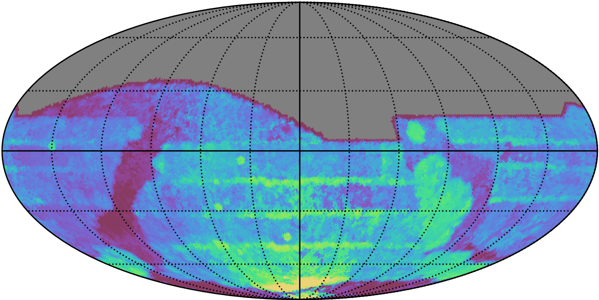
roll_uniform_eh_acc0.5_mjdp0_v3.4_10yrs All sky all bands: Median Season Length
