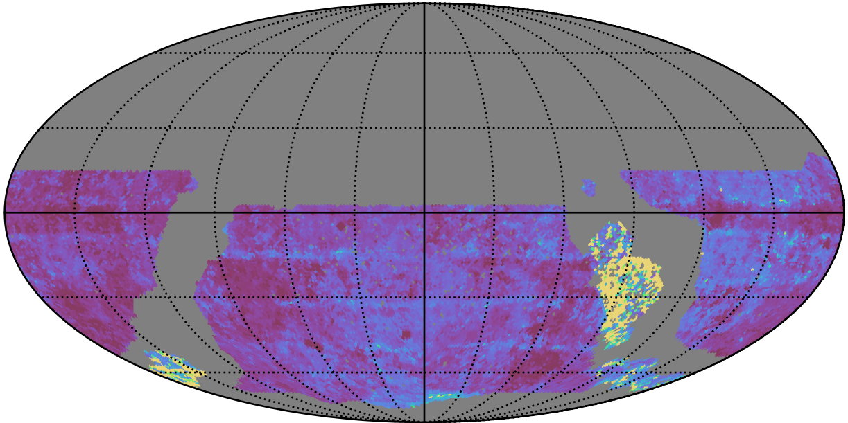
roll_uniform_eh_acc0.5_mjdp0_v3.4_10yrs WFD u band: Median Inter-Night Gap
