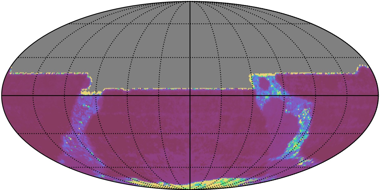
roll_uniform_eh_acc0.5_mjdp0_v3.4_10yrs All sky y band: Median Inter-Night Gap
